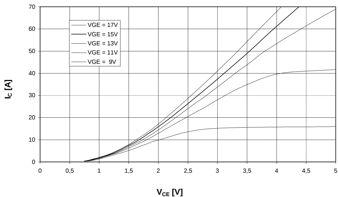
Output characteristic Inverter (typical)
