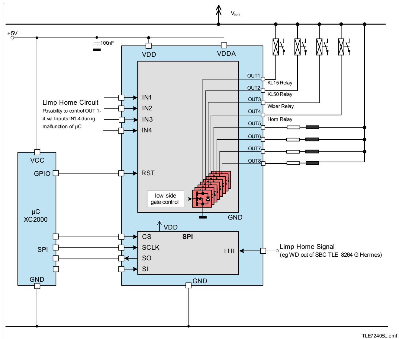
Figure 13 Application Diagram
