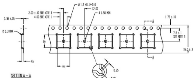
Figure 16: Carrier Tape Outline Drawing
