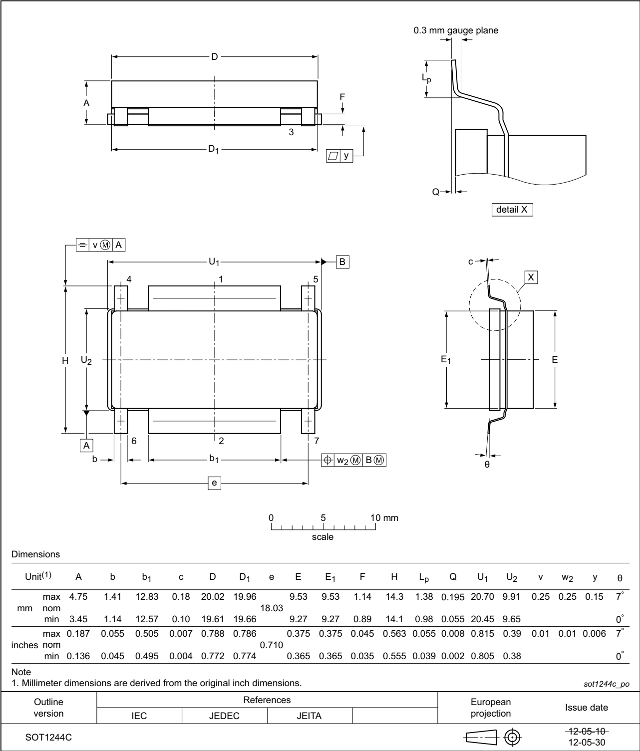
Fig 11. Package outline SOT1244C
