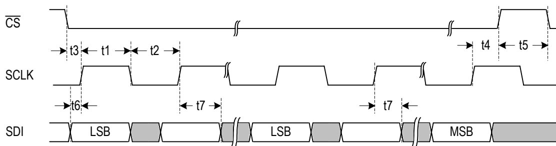
Figure-30 Serial Interface Write Timing
