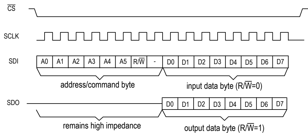
Figure-20 Serial Microcontroller Interface Function Timing
