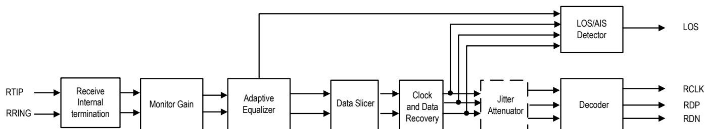
Figure-7 Receive Path Function Block Diagram
