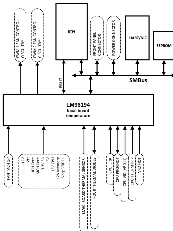
Figure 1. Workstation Management
