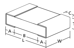
Wrap-around terminations (3 faces)
