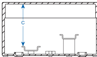
C) from top of mounting rail NS 35 (mounted on base standoffs)
