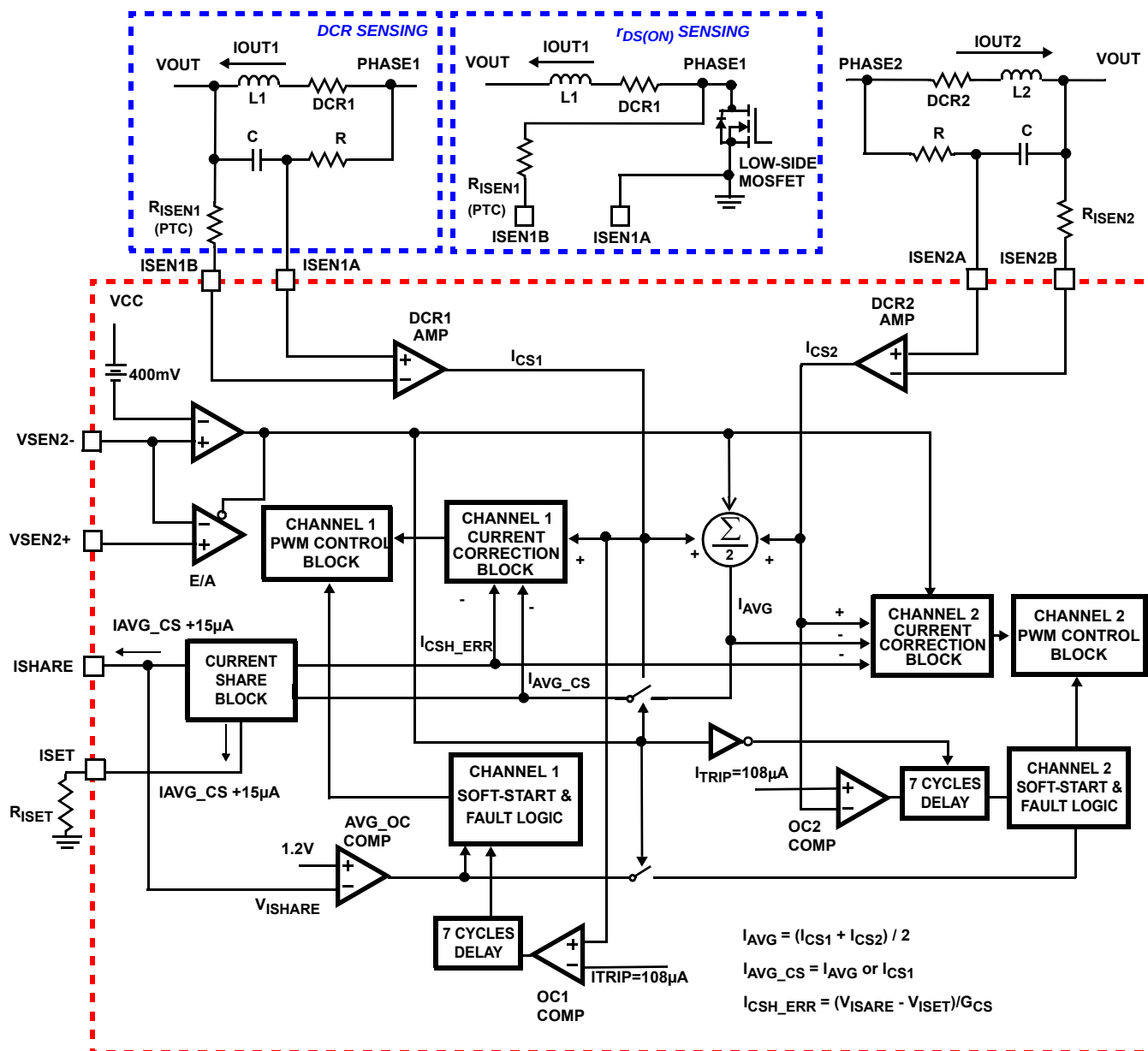
FIGURE 23. SIMPLIFIED CURRENT SAMPLING AND OVERCURRENT PROTECTION
