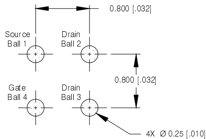
RECOMMENDED FOOTPRINT
