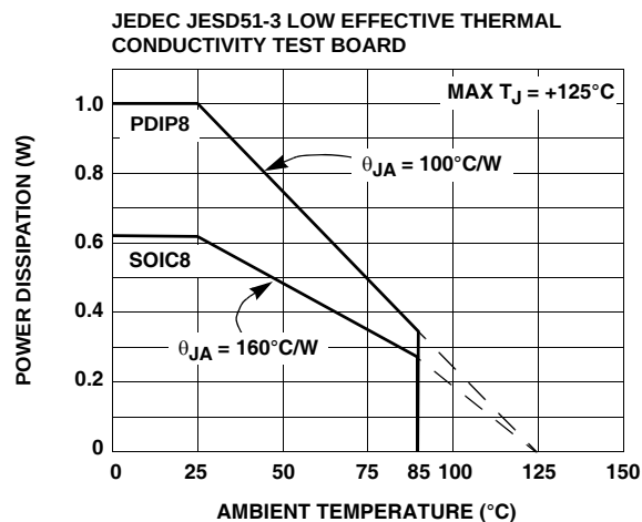
FIGURE 1. PACKAGE POWER DISSIPATION vs AMBIENT TEMPERATURE
