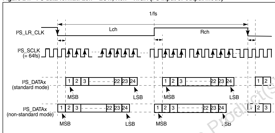
Figure 24. I 2 S data format: Lch = LOW, Rch = HIGH (I 2 S input or output mode)
