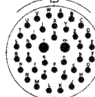
20-39 37 NO.20 2 NO.16 CONTACTS
