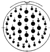
22-41 27 NO.20 14 NO.16 CONTACTS
