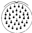
22-41 27 NO.20 14 NO.16 CONTACTS
