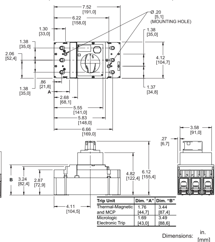
Figure 19: Rotary Handle Detail (PowerPact J-Frame Circuit Breaker)
