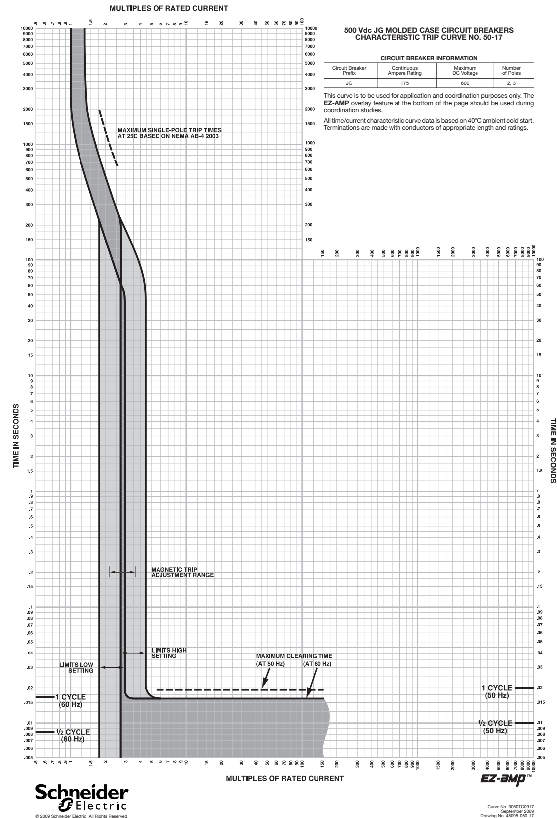
Figure 64: J-Frame 175 A (JG) 500 Vdc Thermal-Magnetic Trip
