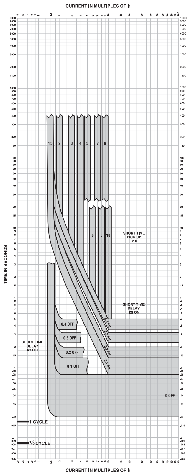
Figure 100: Micrologic 5.3A/5.3E/6.3A/6.3E Electronic Trip Unit Short Time Trip Curve
