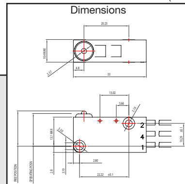
COMMON (black) 1 2 4 NORMALLY CLOSED (grey) NORMALLY OPEN (blue)
