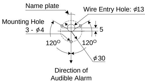
Mounting Dimensions
