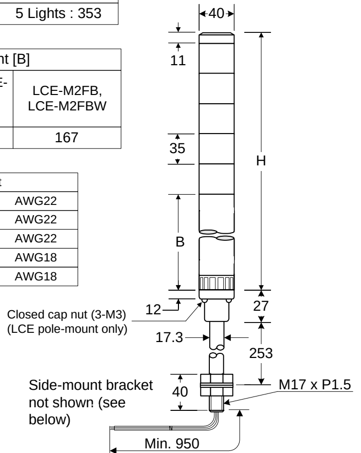
Pole Mount
