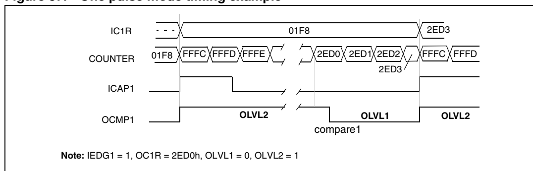
Figure 57. One pulse mode timing example
