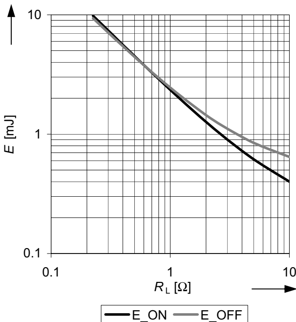
Figure 34 Typical switch ON energy E_{ON} and switch OFF energy E_{OFF} as a function of the load resistance R_L V_S = 13.5V , T_j = 25^\circ C
