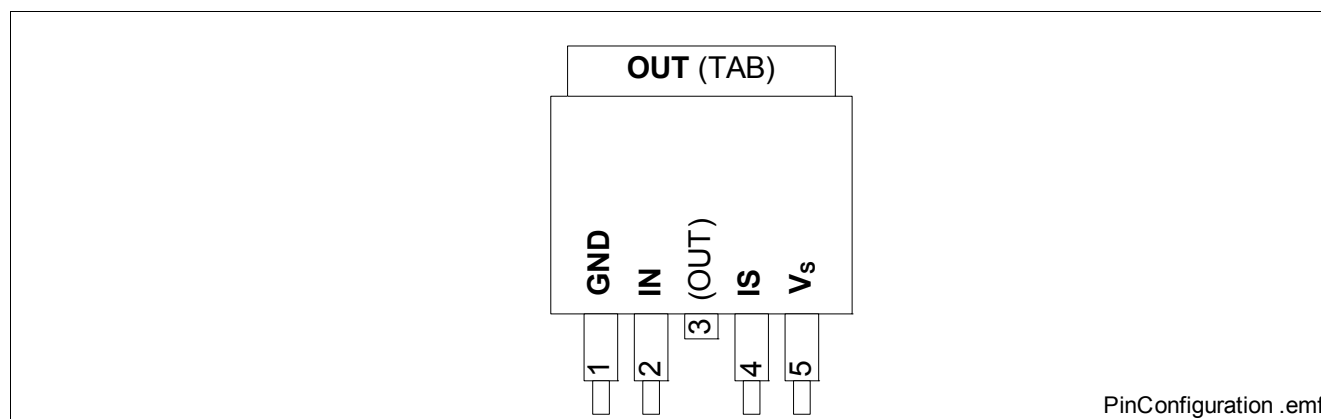
Figure 2 Pin Configuration
