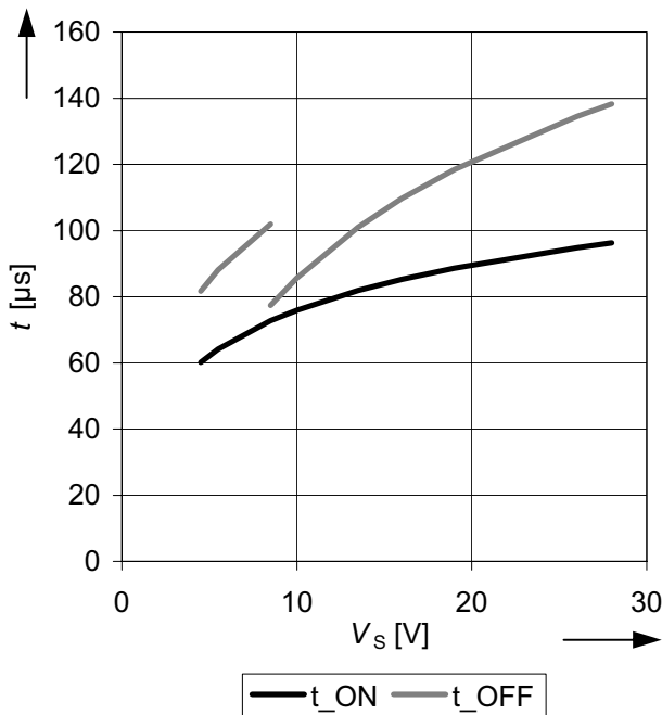
Figure 32 Typical turn ON time t_{ON} and turn OFF time t_{OFF} as a function of the supply voltage V_S T_j = 25^\circ C , R_L = 1\Omega
