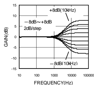
Fig.12 Treble Gain - Frequency
