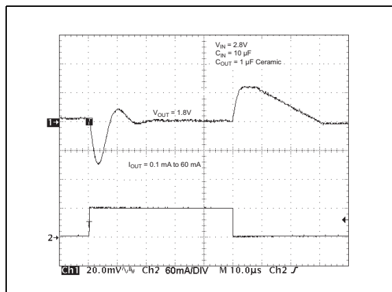
FIGURE 2-23: Load Transient Response.
