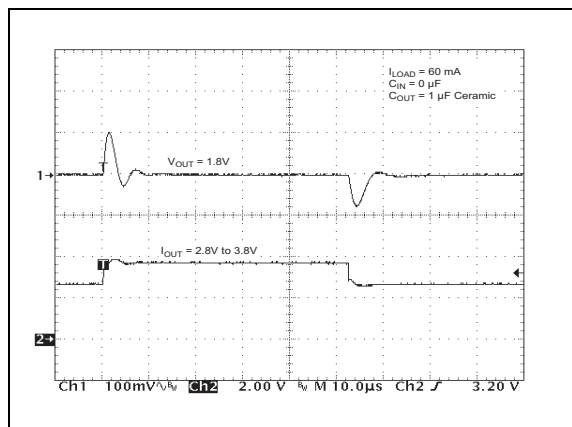
FIGURE 2-24: Line Transient Response.
