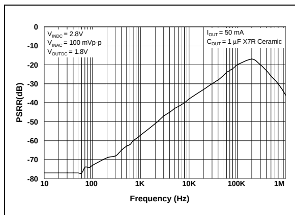
FIGURE 2-19: Power Supply Rejection Ratio vs. Frequency.
