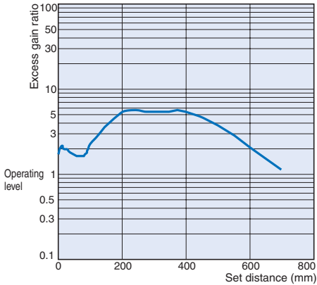
E3T-SR3□ + E39-R37 (Provided)
