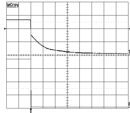
Turn-off at I_o=20A resistive load at T_{Pcb}=+25^\circ C , V_{in}=53V . Turn-off enabled by disconnecting V_{in} . Bottom trace: output voltage (0.5 V/div.). Top trace: input voltage (20 V/div.). Time scale: 5 ms/div.
