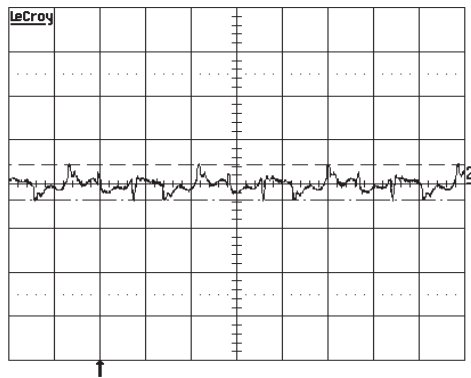
Output voltage ripple (50mV/div.) at T_{Pcb}=+25^\circ C , V_{in}=53V , I_o=20A resistive load with C=10\mu F tantalum and 0.1\mu F ceramic capacitors. Band width=20MHz. Time scale: 2μs / div.
