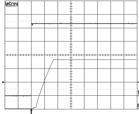
Start-up at I_o=20A resistive load at T_{Pcb}=+25^\circ C , V_{in}=53V . Start enabled by connecting V_{in} . Top trace: input voltage (10 V/div.). Bottom trace: output voltage (0.5 V/div.). Time scale: 5 ms/div.
