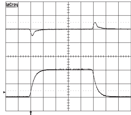
Output voltage response to load current step-change (5-15-5 A) at T_{Pcb}=+25^\circ C , V_{in}=53V . Top trace: output voltage (200mV/div.). Bottom trace: load current (5 A/div.) Time scale: 0.1 ms/div.
