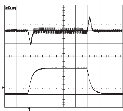
Output voltage response to load current step-change (5-15-5 A) at T_{Pcb}=+25\text{ }^{\circ}C , V_{in}=53\text{ V} . Top trace: output voltage (100mV/div.). Bottom trace: load current (5 A/div.). Time scale: 0.1 ms/div.
