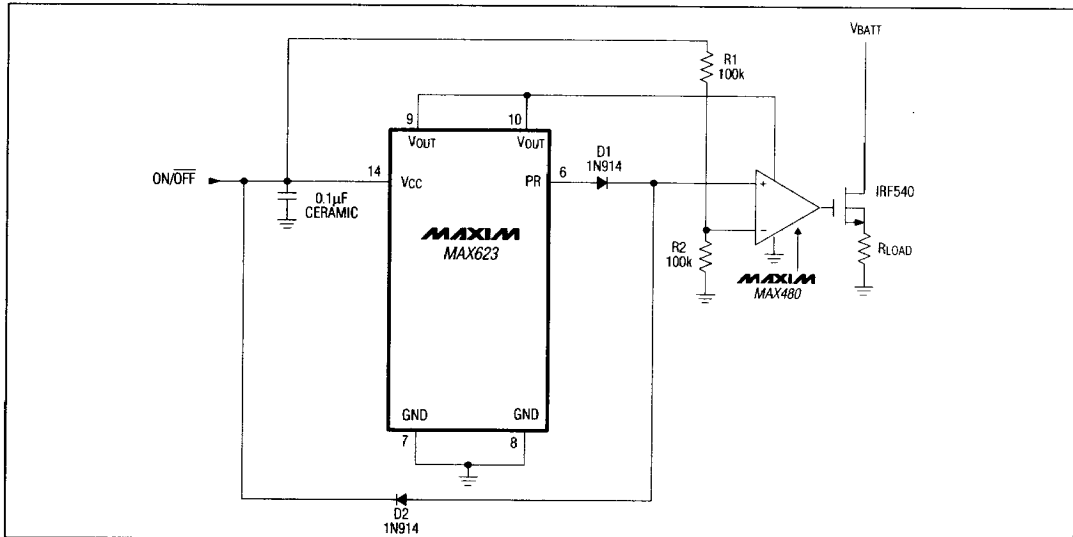
Figure 3. Single-Load Switch
