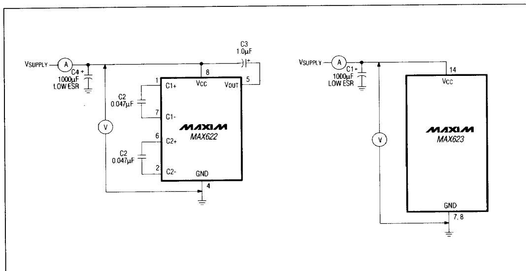
Figure 2. MAX622/MAX623 Quiescent Supply-Current Test Circuits
