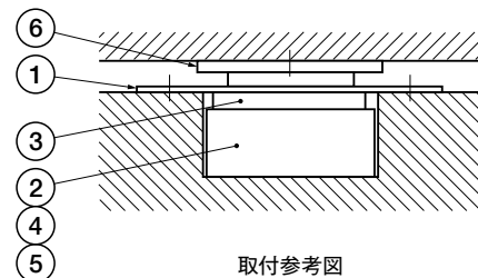
取付参考図 Reference Layout for Installation
