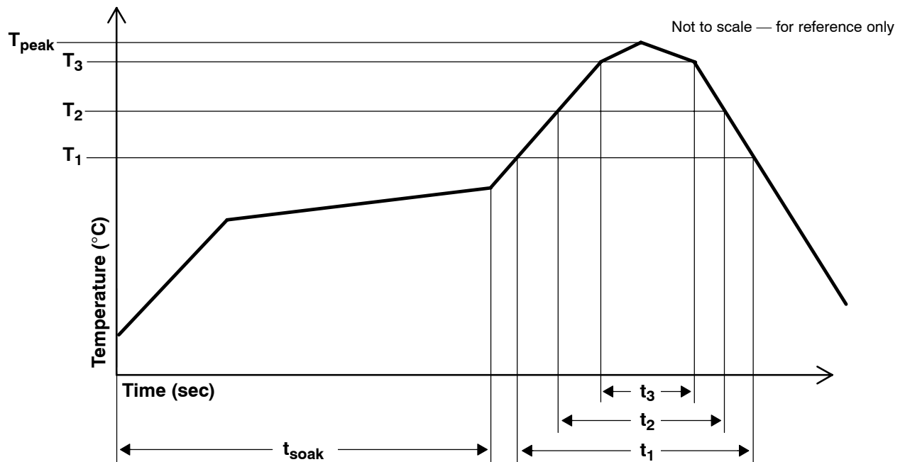
Figure 10. TSL230RD Solder Reflow Profile Graph
