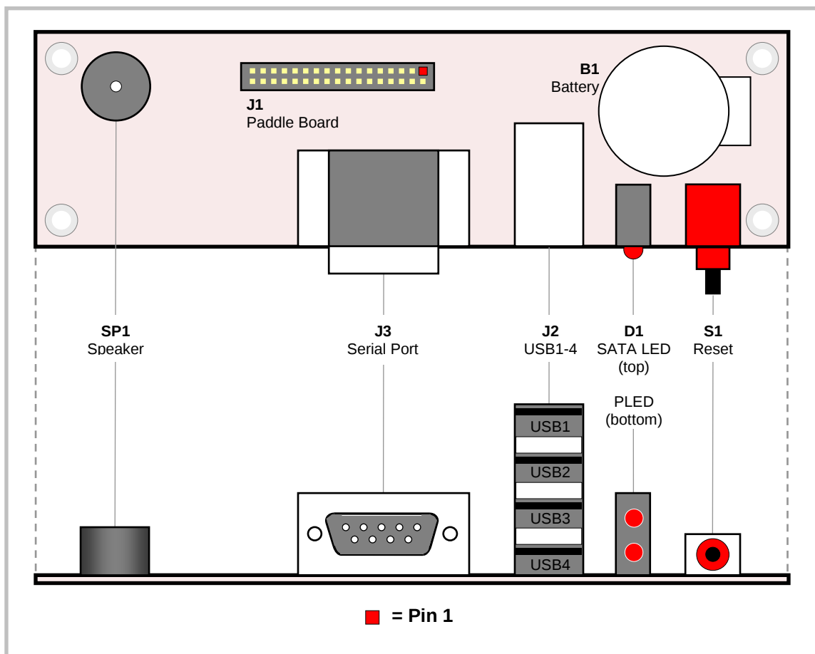
Figure 9. VL-CBR-3406 Connector Locations
