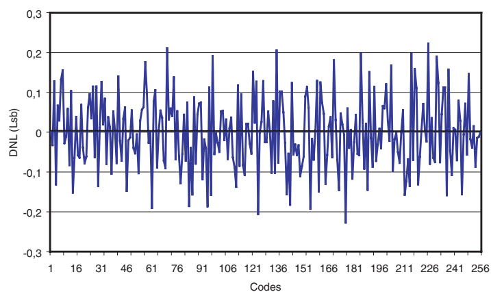
Figure 9-3. Typical DNL (Fs = 50 Msps, Fin = 1 MHz, Saturated Input)
