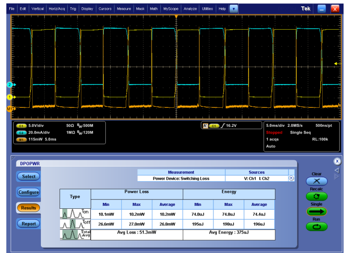
Switching Loss measurements. Automated power measurements enable quick and accurate analysis of common power parameters.
