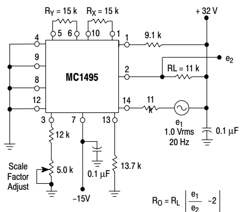
Figure 8. Output Resistance
