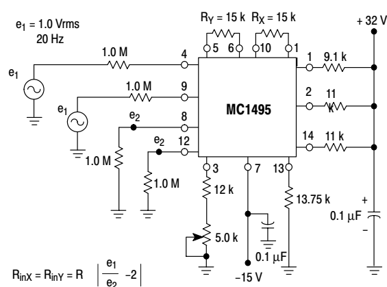
Figure 7. Input Resistance
