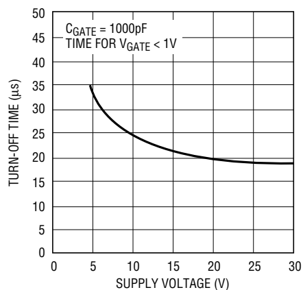
Turn-OFF Time
