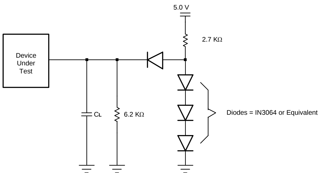
Figure 7. Test Setup
