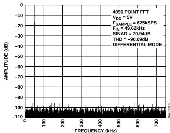
Figure 6. FFT @ V_{DD} = 5V
