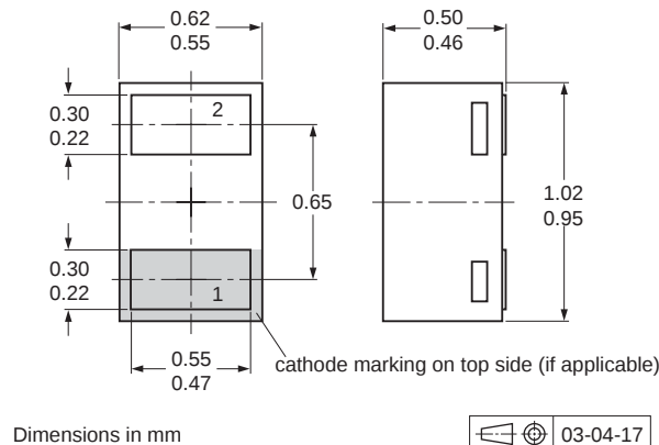
Fig 12. Package outline PESD5V0V1BL (SOD882)
