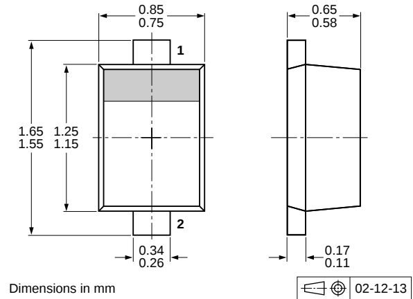
Fig 11. Package outline PESD5V0V1BB (SOD523/SC-79)
