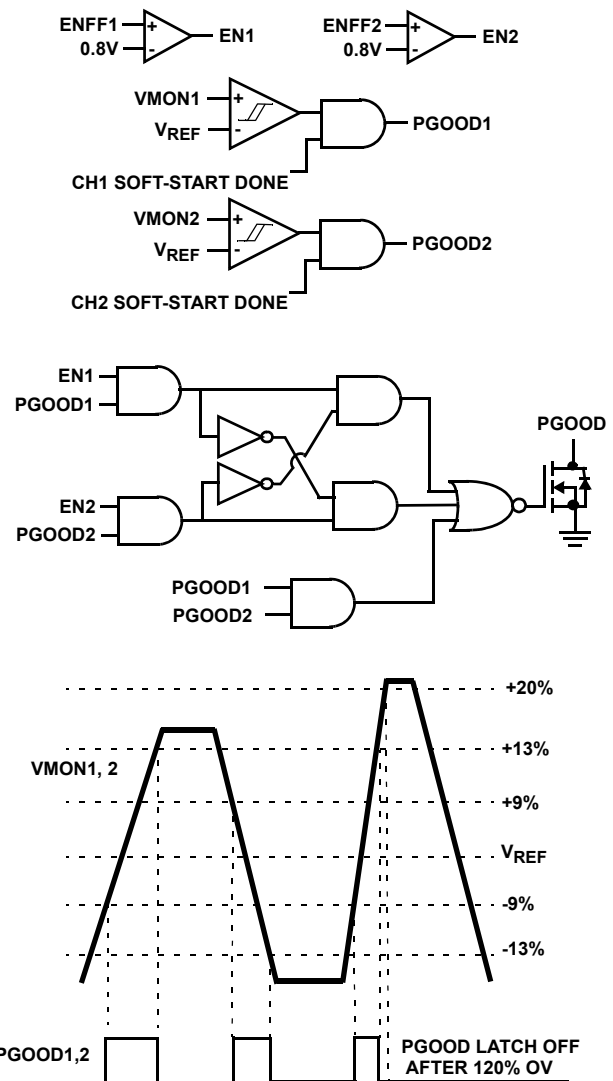
FIGURE 29. POWER-GOOD THRESHOLD WINDOW
