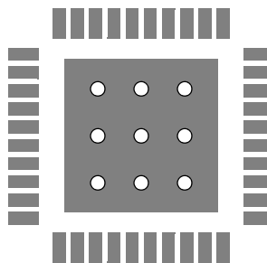
FIGURE 48. PCB VIA PATTERN
