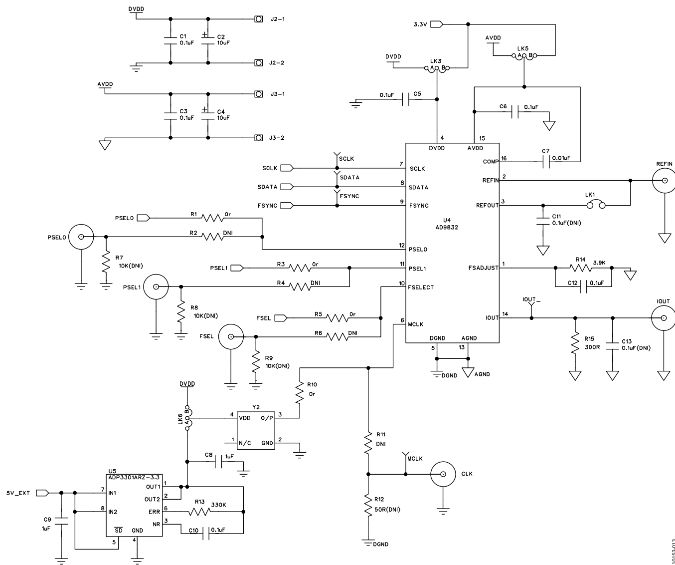
Figure 13. AD9832 Schematic Part A
