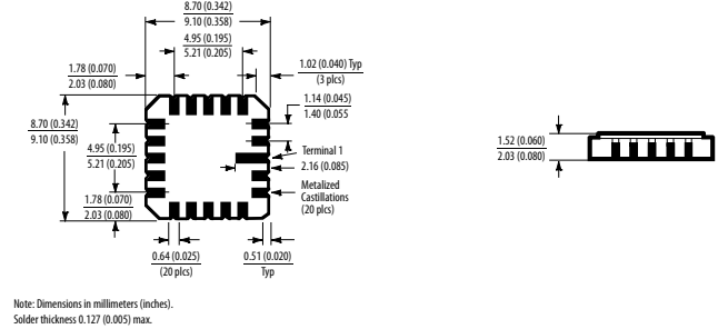
20 Terminal LCCC Surface Mount (2 Channel)
