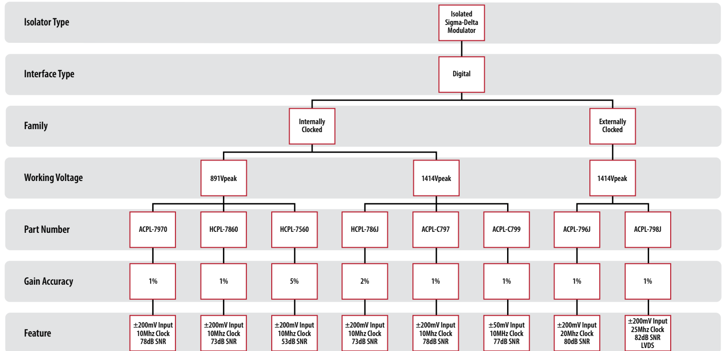
Isolated Sigma-Delta Modulator Product Tree
