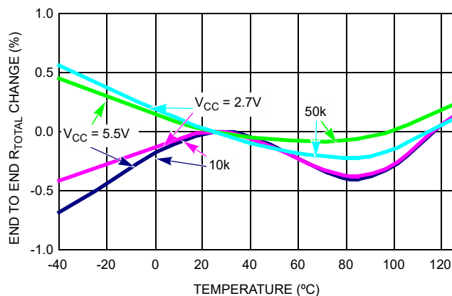
Figure 12. End-to-End R_{TOTAL} % Change vs Temperature
