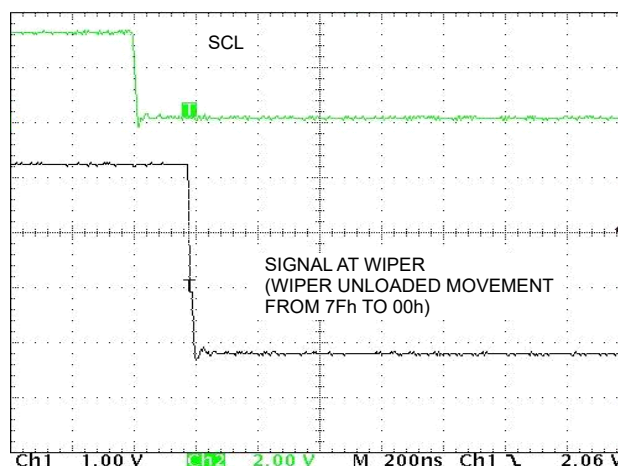
Figure 17. LARGE SIGNAL SETTLING TIME
