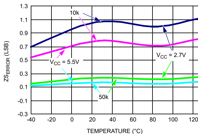
Figure 8. ZS_{ERROR} vs Temperature
