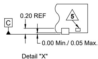
Detail "X"
