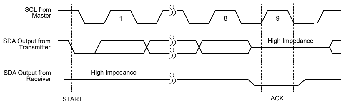
Figure 20. Acknowledge Response from Receiver
