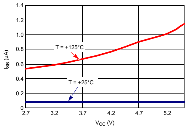
Figure 5. Standby I_{CC} vs V_{CC}
