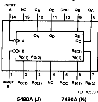
Dual-In-Line Package
