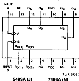
Dual-In-Line Package
