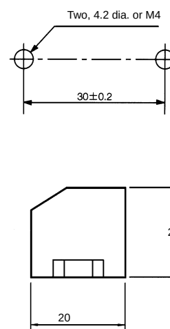
Mounting Holes
