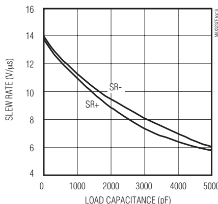
MAX3246E SLEW RATE vs. LOAD CAPACITANCE
