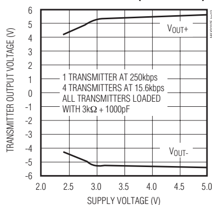
MAX3237E TRANSMITTER OUTPUT VOLTAGE vs. SUPPLY VOLTAGE (MBAUD = GND)
