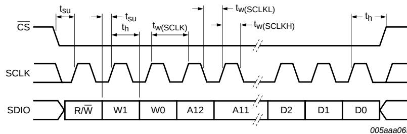
Fig 5. SPI timing
