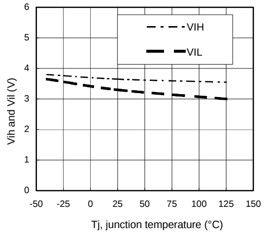
Figure 6 – V_{ih} and V_{il} (V) Vs T_j ( ^{\circ}C )
