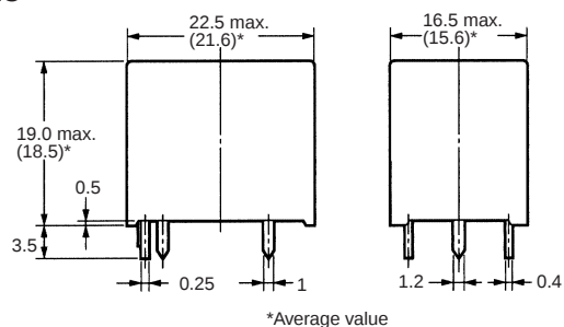
Terminal Arrangement/Internal Connections (Bottom View)
