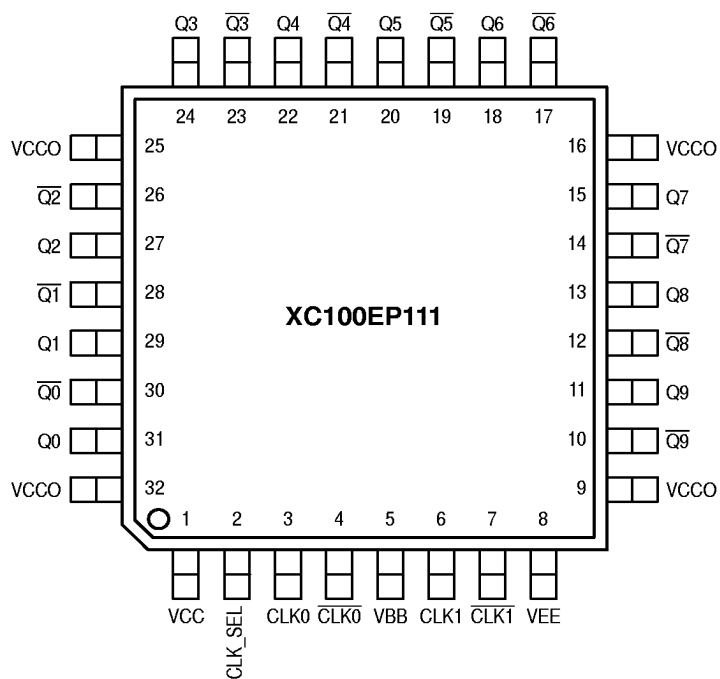
Figure 1. 32-Lead LQFP Pinout (Top View)
