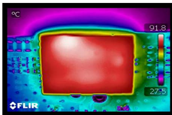
Figure 20 — Thermal Image ( V_{IN} = 28V , I_{OUT} = 10A , CR, OLFM Evaluation PCB)
