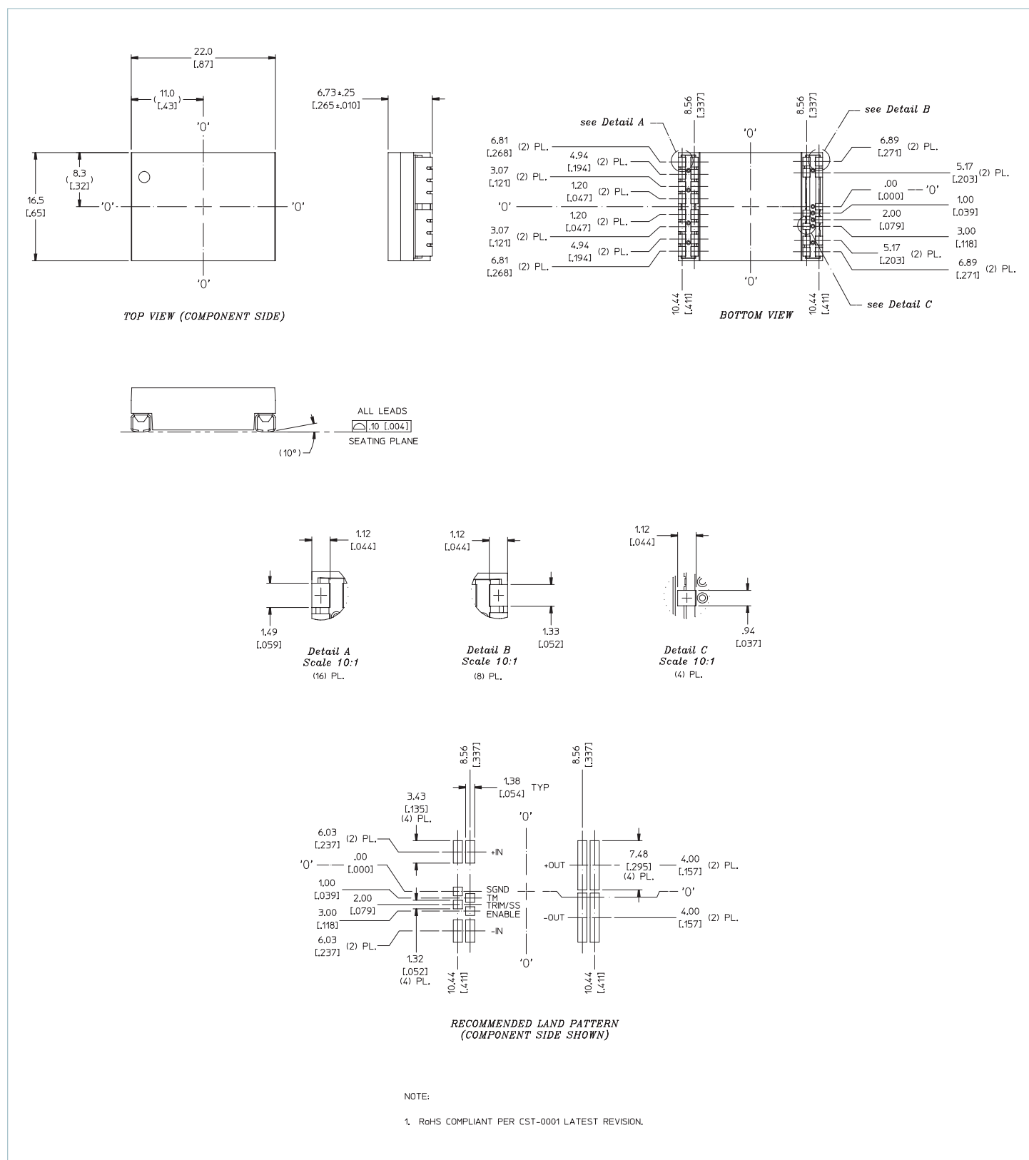
Figure 43 — Package Outline &amp; Recommended PCB Land Pattern
