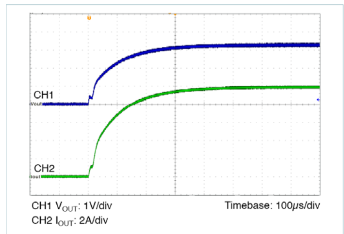
Figure 6 — Start Up, C_{REF} = 0 ( V_{IN} = 28\text{V} , I_{OUT} = 10\text{A} , CR, C_{OUT} = 6 \times 10\mu\text{F} X7R Ceramic)
