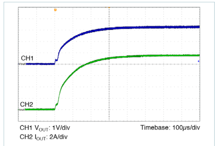
Figure 5 — Start Up, C_{REF} = 0 ( V_{IN} = 16\text{V} , I_{OUT} = 10\text{A} , CR, C_{OUT} = 6 \times 10\mu\text{F} X7R Ceramic)
