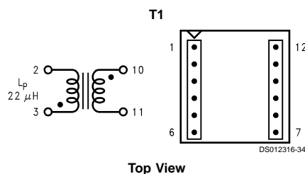
FIGURE 19. Coilcraft Q4435-B (Surface Mount)
