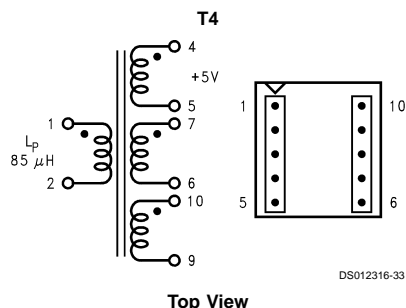
FIGURE 18. Coilcraft Q4344-B
