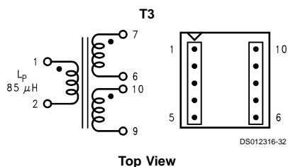
FIGURE 17. Coilcraft Q4343-B
