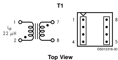
FIGURE 15. Coilcraft Q4434-B
