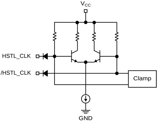
Figure 2. Simplified HSTL Input Stage
