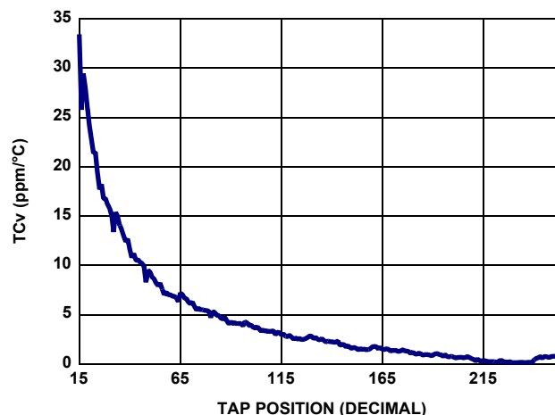
FIGURE 10. 100k TCv vs TAP POSITION
