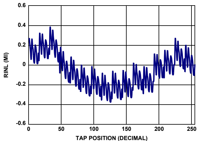
FIGURE 6. 10k RINL vs TAP POSITION, V_{CC} = 5V
