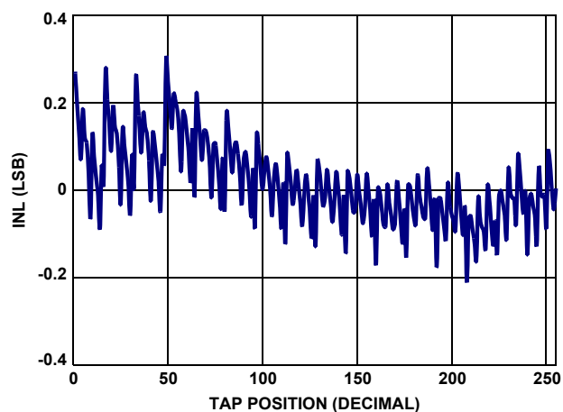
FIGURE 4. 10k INL vs TAP POSITION, V_{CC} = 5V
