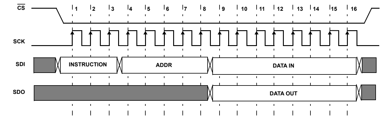
FIGURE 24. TWO BYTE READ INSTRUCTION
