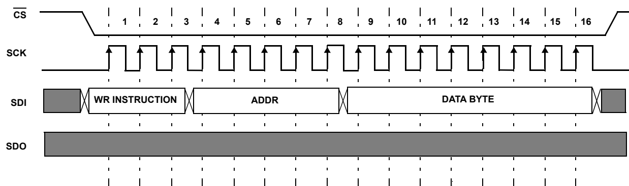
FIGURE 20. TWO BYTE WRITE SEQUENCE
