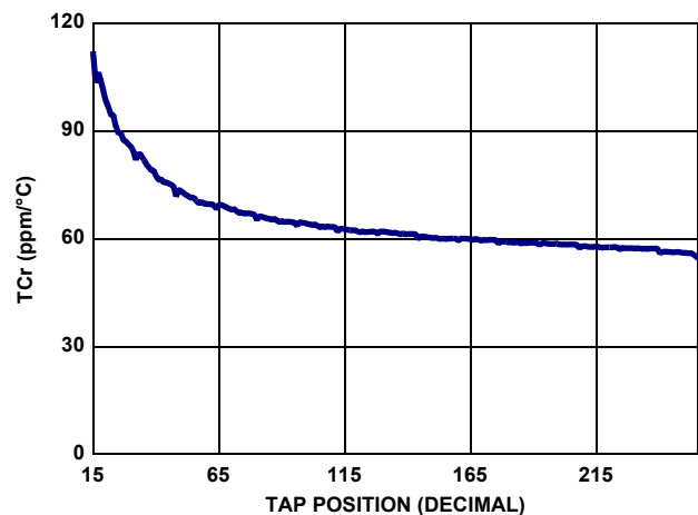
FIGURE 11. 100k TCr vs TAP POSITION
