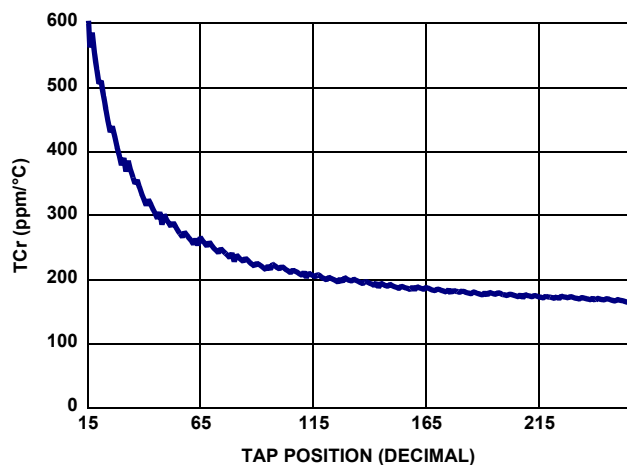
FIGURE 9. 10k TCr vs TAP POSITION
