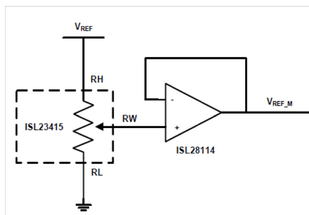
FIGURE 2. V_{\text{REF}} ADJUSTMENT
