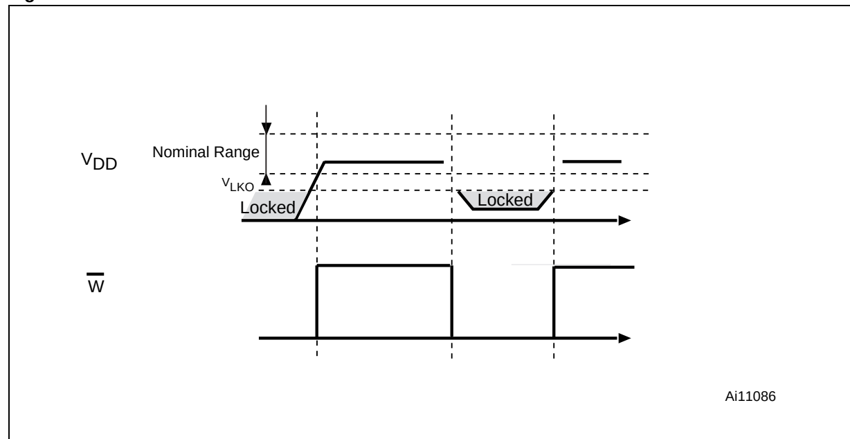
Figure 37. Data Protection
