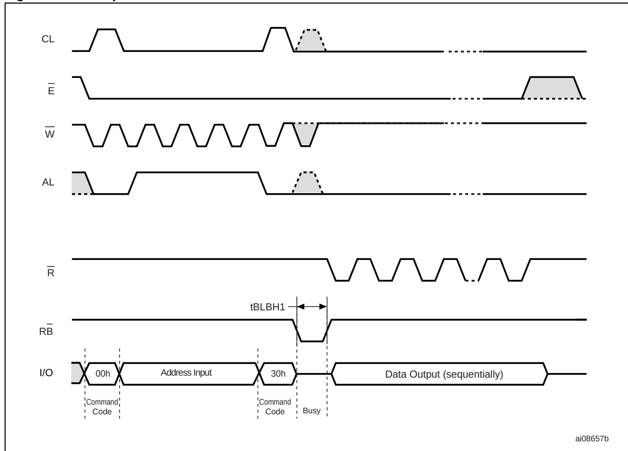
Figure 8. Read Operations
