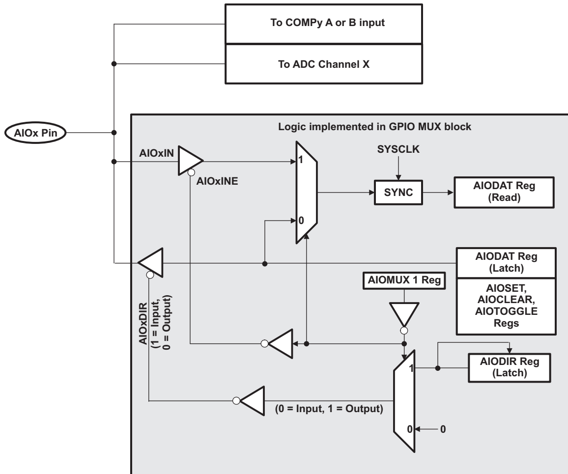
Figure 6-29. AlOx Pin Multiplexing
